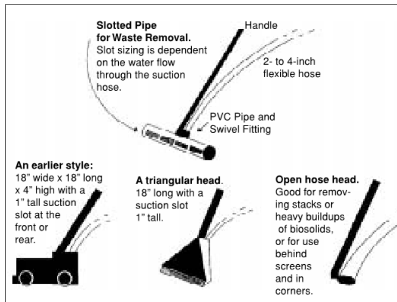
Figure 3-12. Typical Vacuum Removal of Solids (Source: Idaho DEQ, nd)
