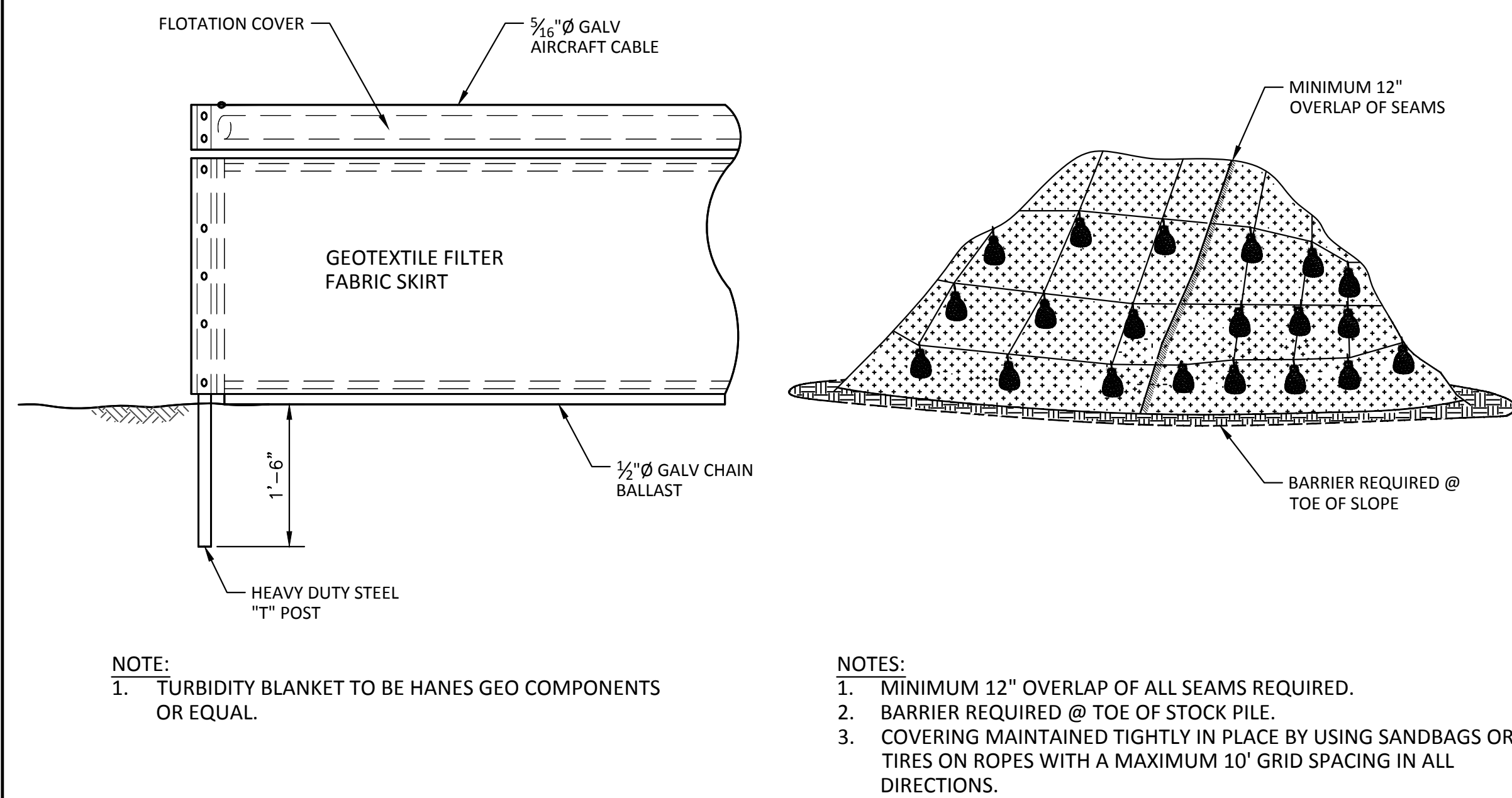
TURBIDITY CURTAIN DETAIL
