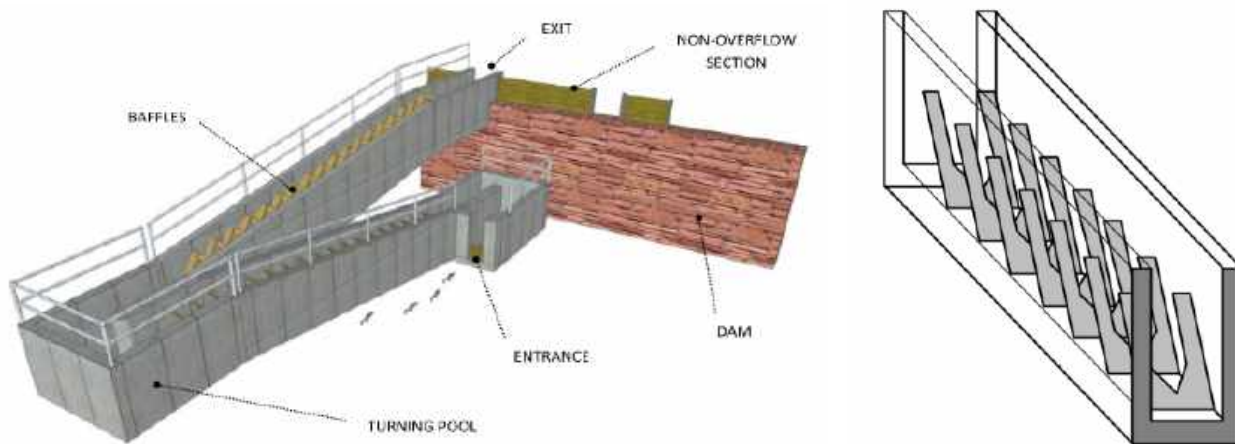
Figure 1. Denil Fishway Schematics (Left Source: USFWS, 2017; Right Source: NRCS, 2007 )
