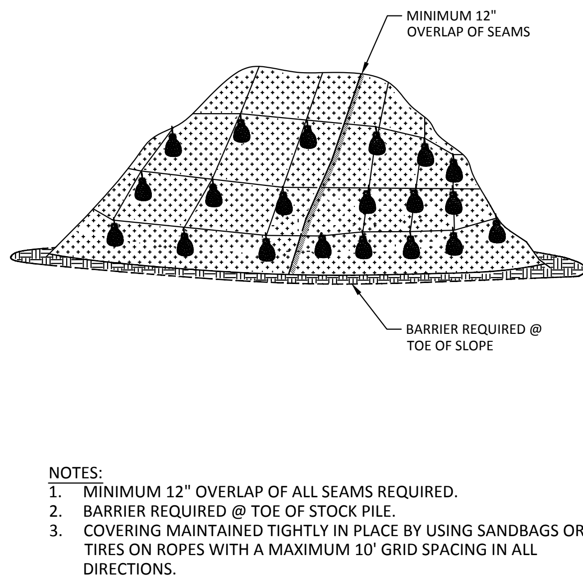
PLASTIC SHEETING DETAIL
