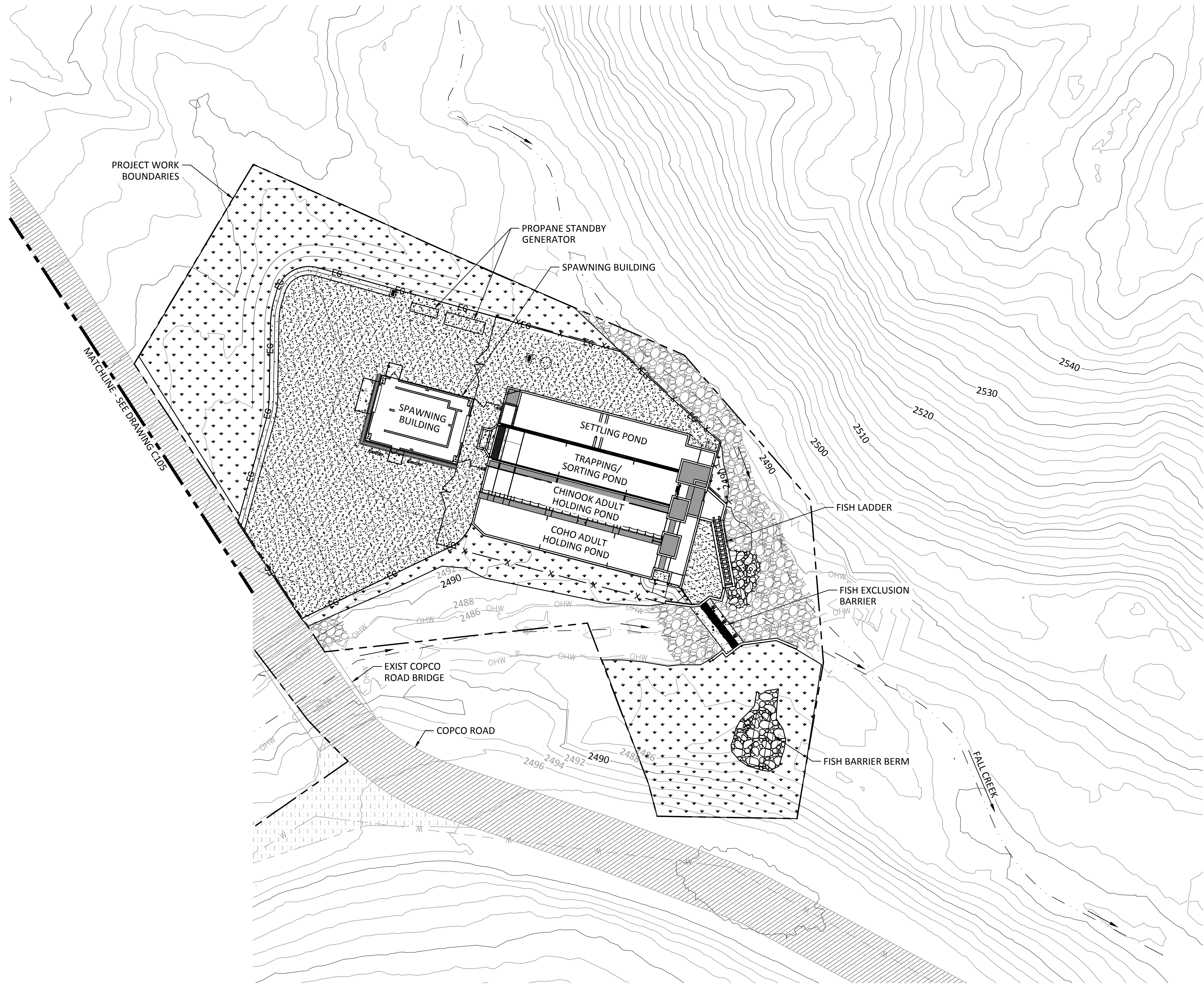
SITE RESTORATION SOUTH PLAN SCALE: 1"= 20'
