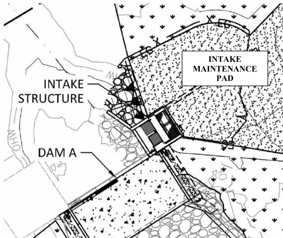
Figure 2-8. FCFH Intake Structure and Dam A Plan View.
