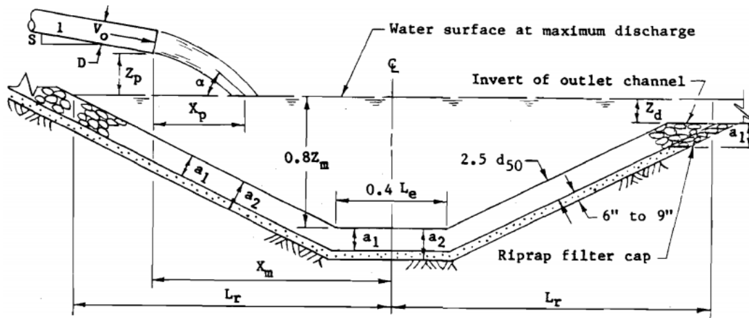
Figure 3. Plunge Pool Definition Sketch (Source; NRCS, 1986)
