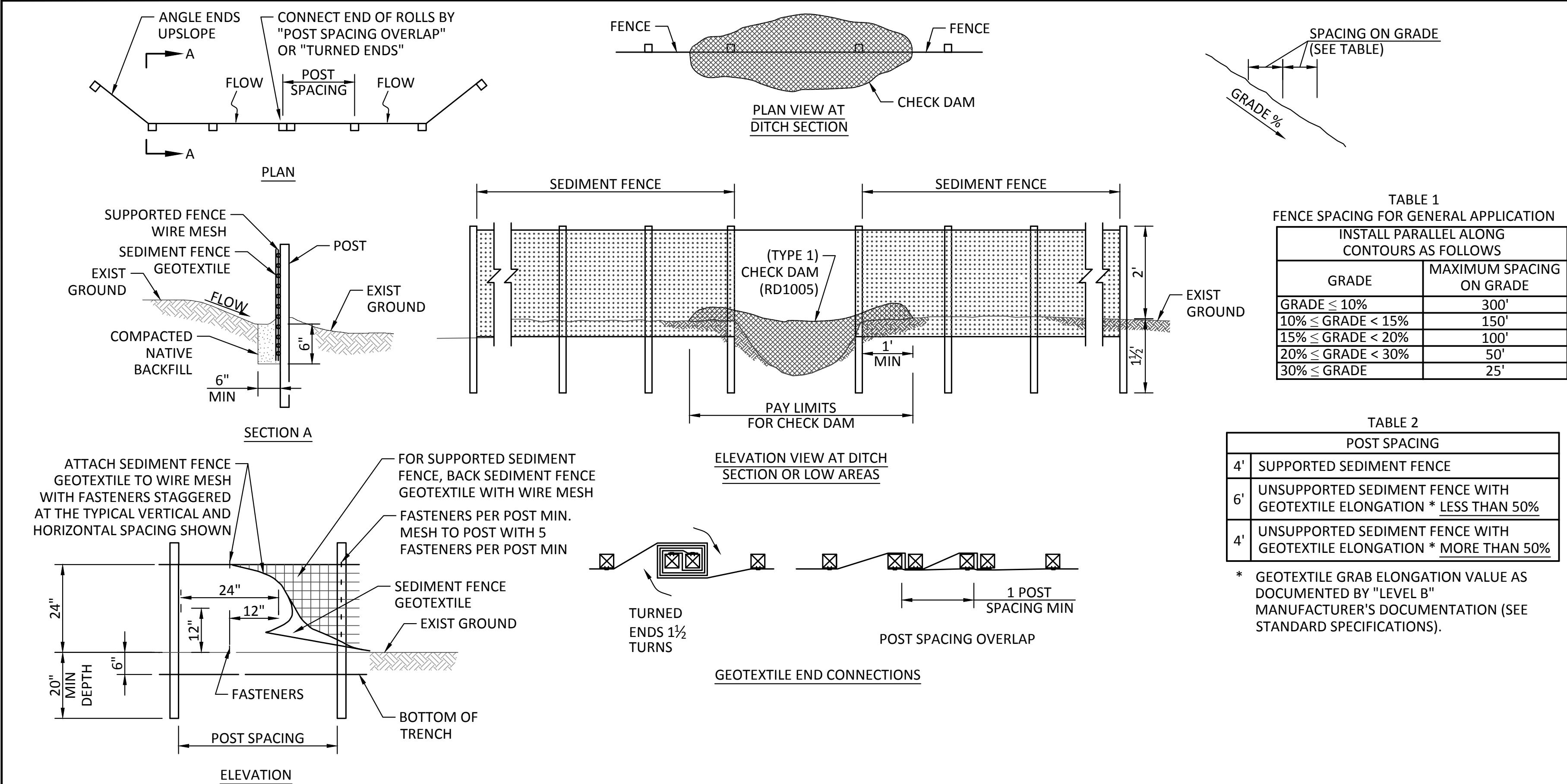
SILT FENCE DETAIL
