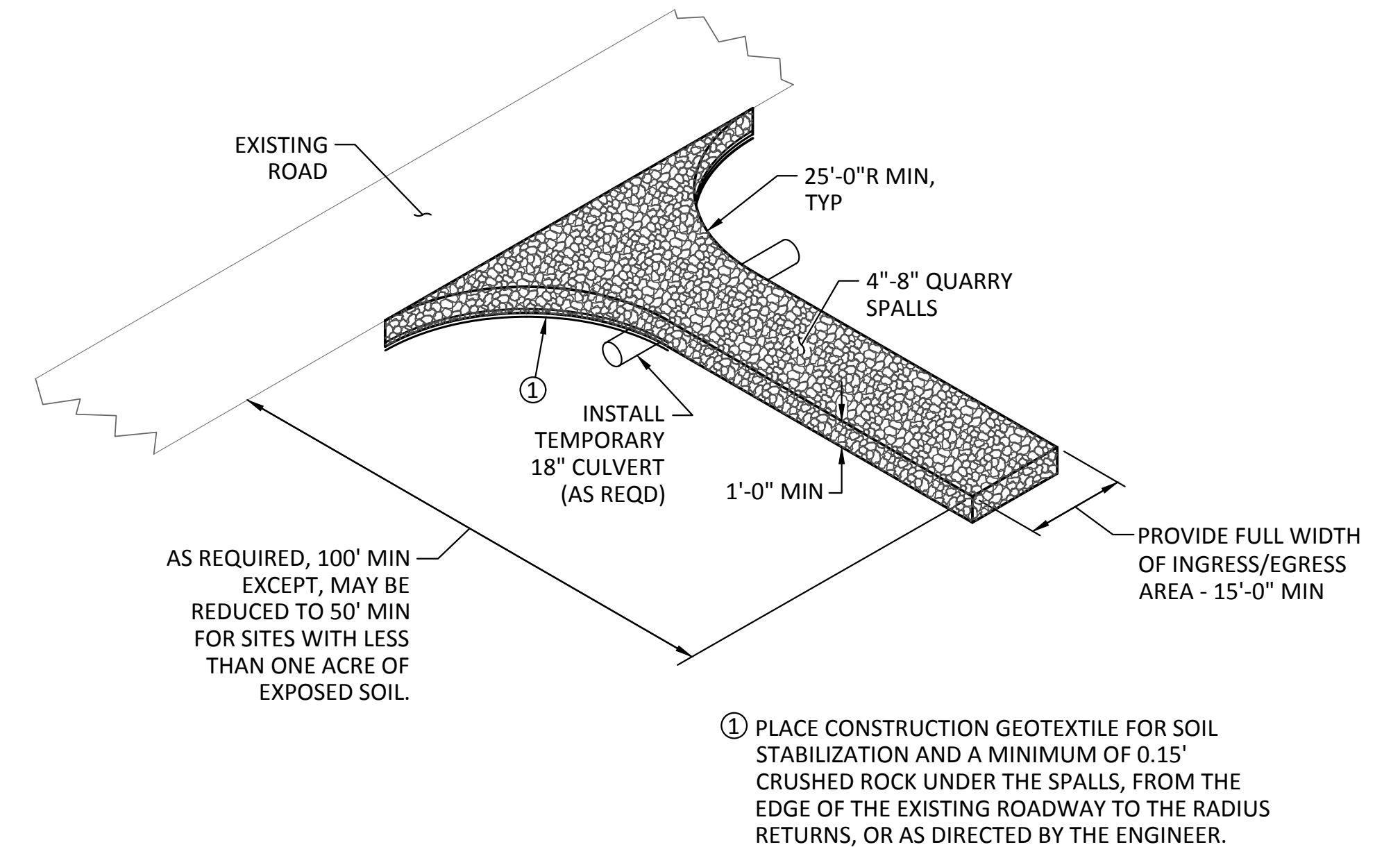
TEMPORARY ENTRANCE
