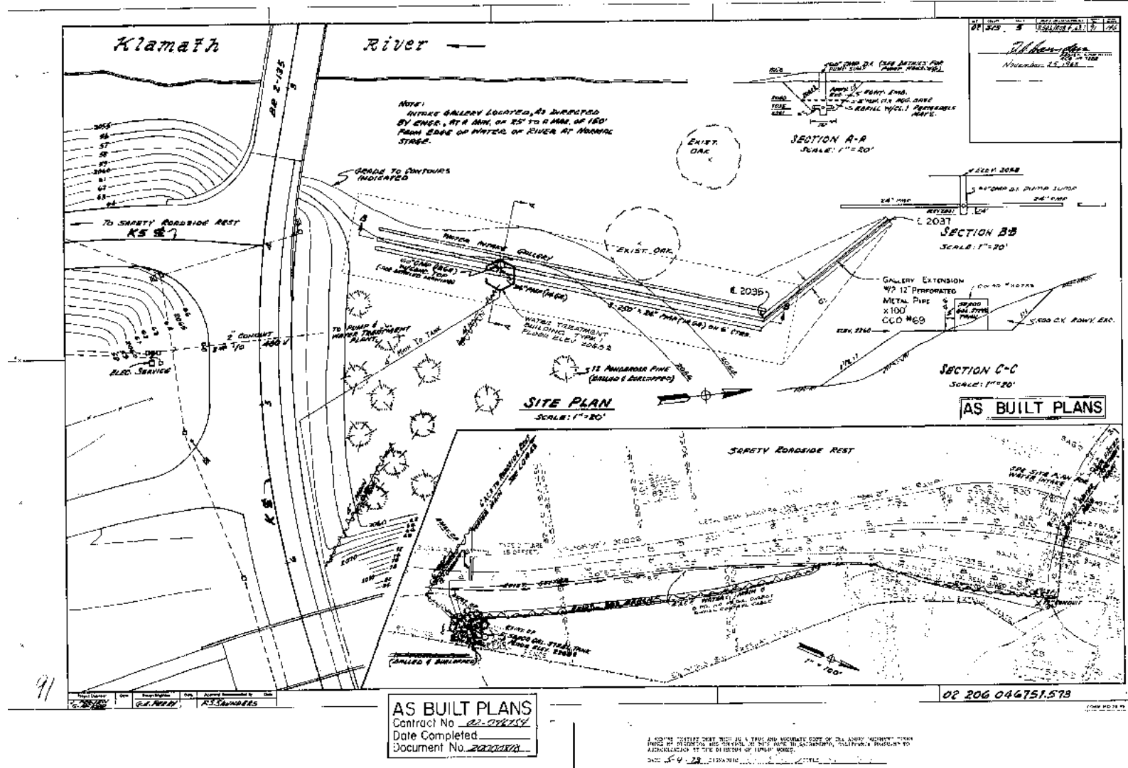
Figure A-1. As-built - Drinking Water System
