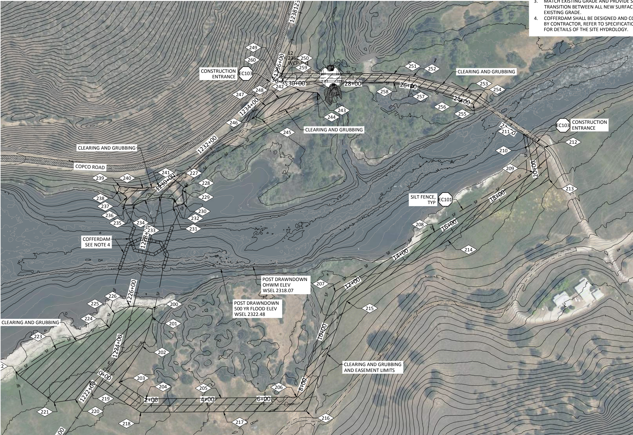
EROSION AND SEDIMENT CONTROL PLAN SCALE: 1"= 100'
