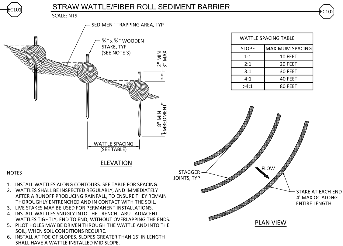
WATTLE SCALE: NTS
