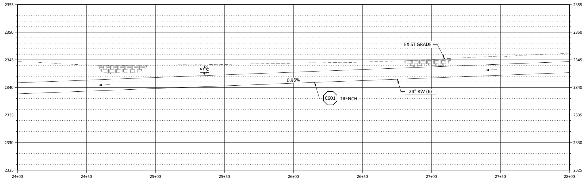
PROFILE SCALE: HORIZ 1"= 20' VERT 1"= 5'
