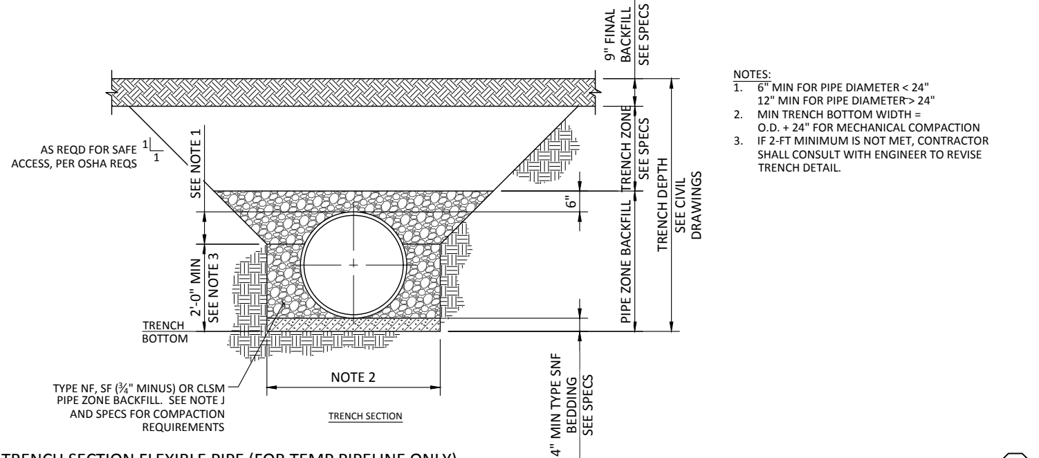
TRENCH SECTION FLEXIBLE PIPE (FOR TEMP PIPELINE ONLY) SCALE: NTS
