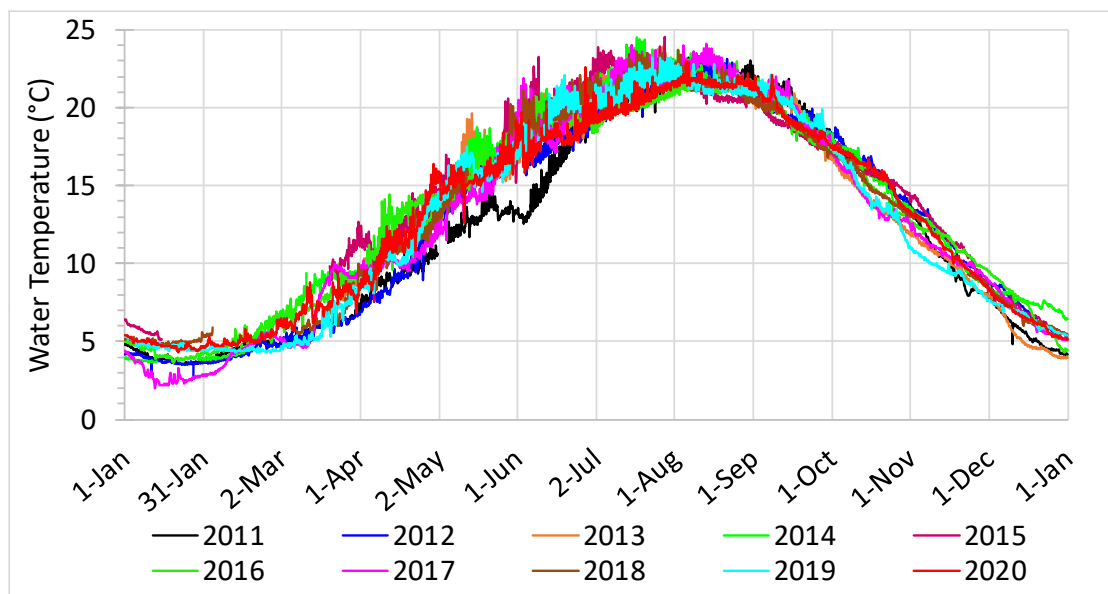
Figure 3.3-6. Hourly water temperatures measured below Iron Gate Dam, 2011–2020 (Source: PacifiCorp, 2012, 2013, 2014, 2015, 2016a, 2017b, 2018, 2019a, 2020a, 2021a)
