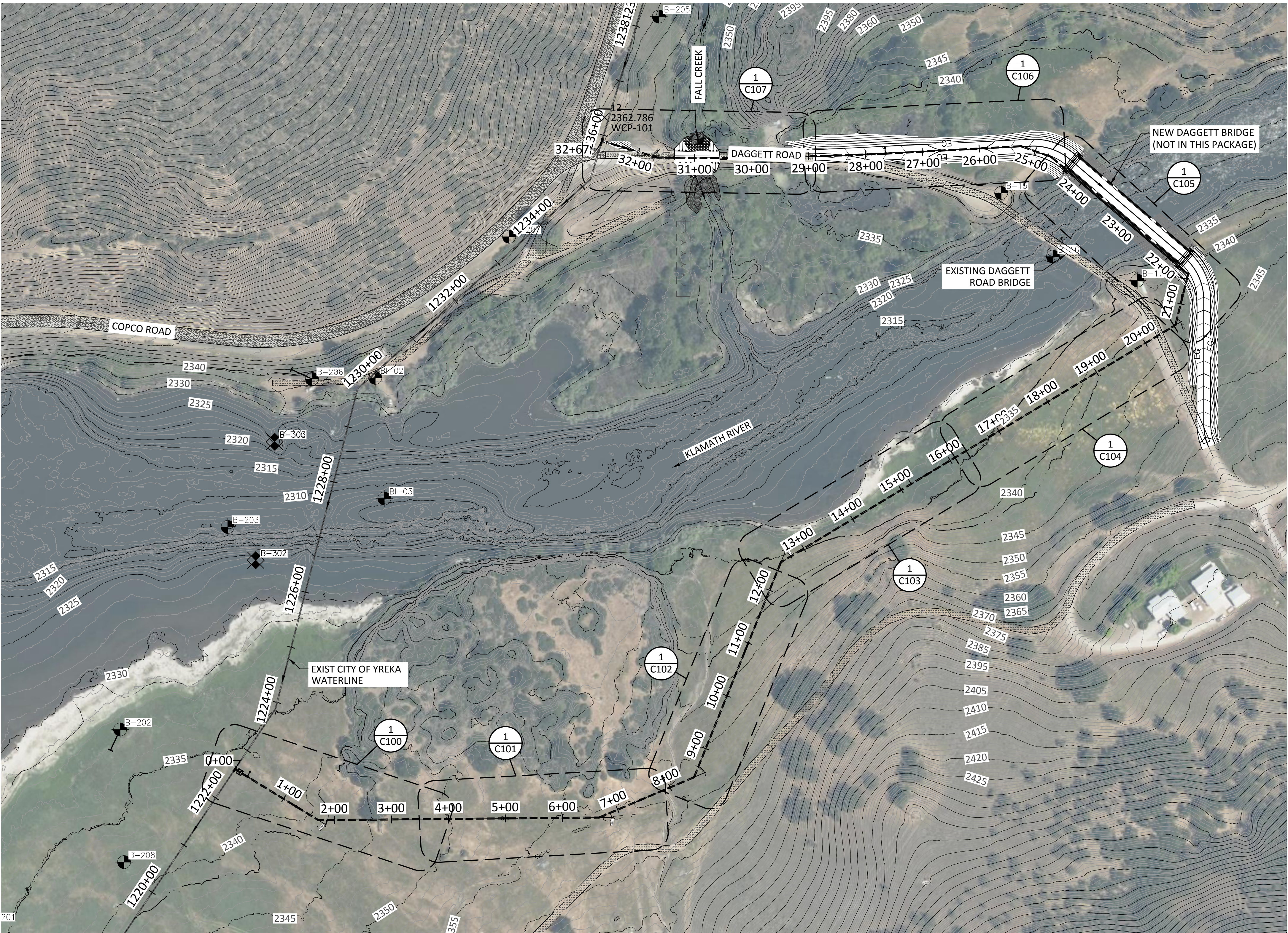
OVERALL SITE PLAN
